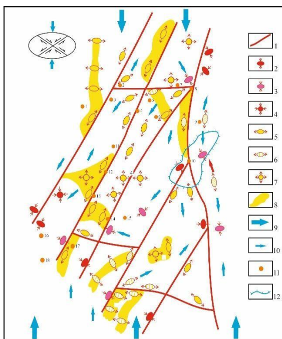
Fig. 2. Scheme of the geodynamic situation of the ore formation period of the Daugiztau ore field. Option 3. (The basis is in m-be 1: 50,000).
